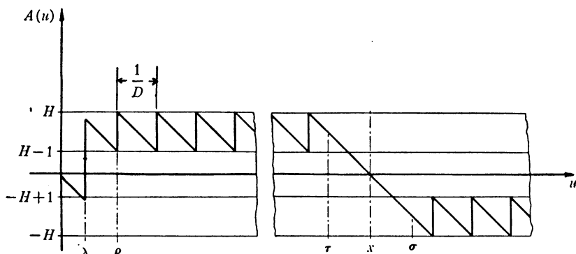
FIG. 1. A function A(u) = \Lambda(u) - Du for which |A(u)| \leq H and |F(x)| > Cx^{4H-2} .
